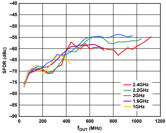
Figure 8. SFDR vs. f_{OUT} over f_{DAC} , Full-Scale Current = 20 mA, Digital Scale = 0 dBFS, Temperature = 25°C
