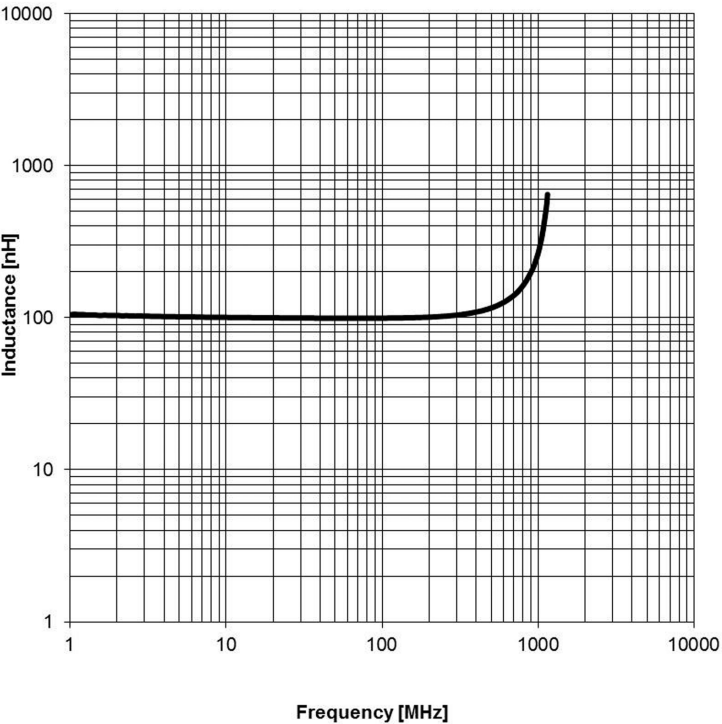
F1 Typical Inductance vs. Frequency Characteristics:
