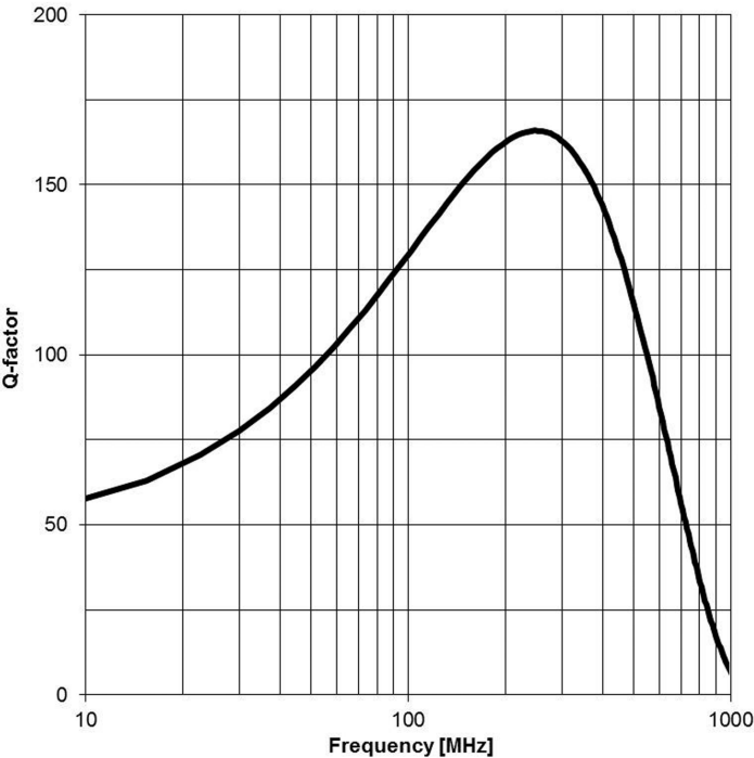
F2 Typical Q-factor vs. Frequency Characteristics:
