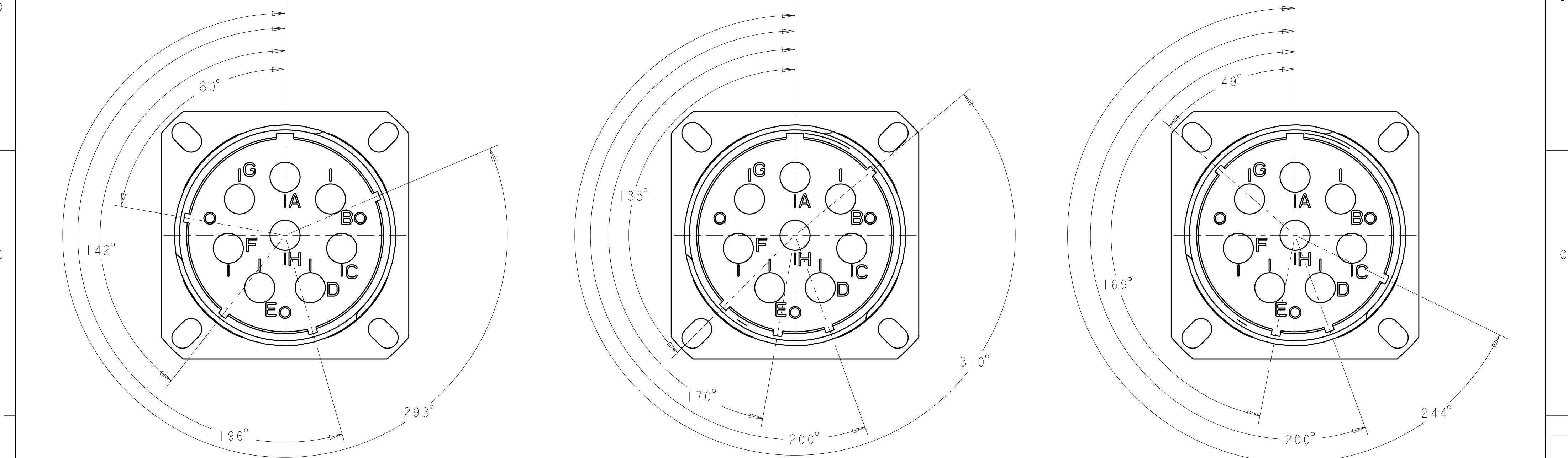
1811927-1 "N" KEY POLARIZATION 1811927-2 "A" KEY POLARIZATION 1811927-3 "B" KEY POLARIZATION
