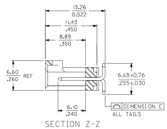
4 CIRCUIT SHOWN
