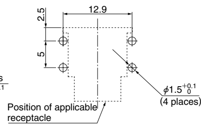
HR12-10R-SP(71) (Stopper plate) (Applicable PCB thickness range 1-2)
