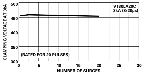
Figure 13 & 14. Typical Repetitive Surge Current Capability of C-III Series MOVs
