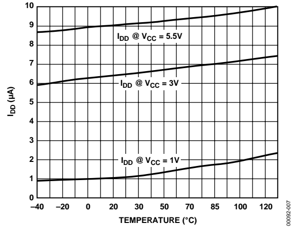
Figure 7. Supply Current vs. Temperature (ADM811L/ADM812L/ADM811M/ADM812M)
