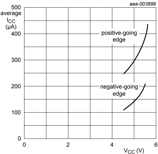
Figure 12. Average additional supply current as a function of V_{CC} for 74HCT132; linear change of V_I between 0.1V_{CC} to 0.9V_{CC} .
