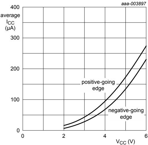
Figure 11. Average additional supply current as a function of V_{CC} for 74HC132; linear change of V_I between 0.1V_{CC} to 0.9V_{CC} .
