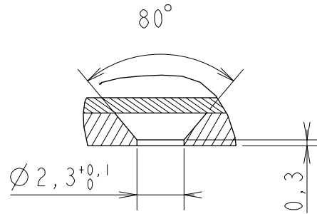
SECTION X-X SCALE 4:1
