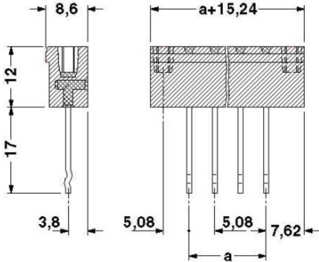
Dimensional drawing
