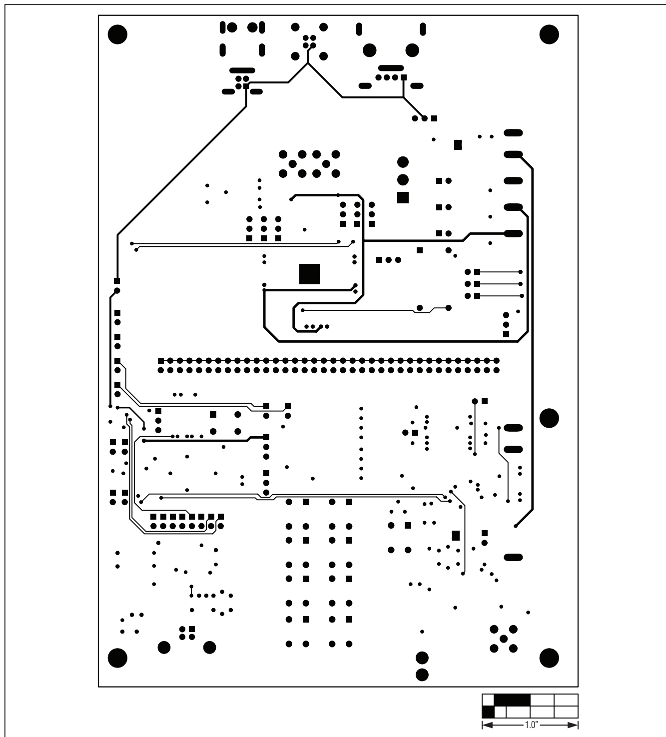
Figure 13. MAX9259 EV Kit PCB Layout—Solder Side
