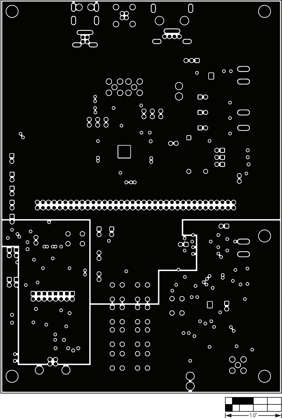
Figure 12. MAX9259 EV Kit PCB Layout—Power Layer 3
