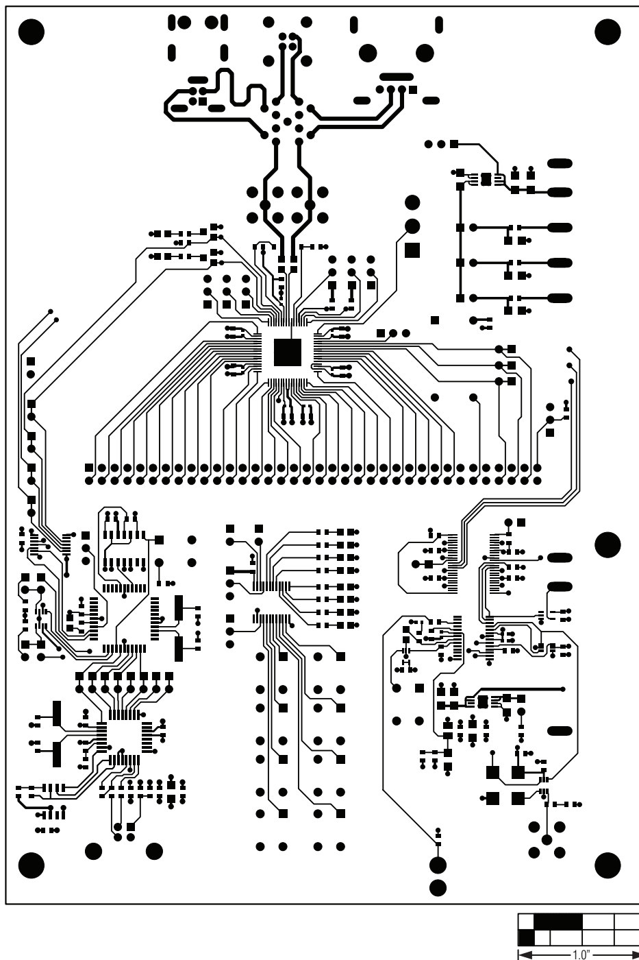
Figure 10. MAX9259 EV Kit PCB Layout—Component Side
