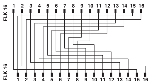
Connection diagram
