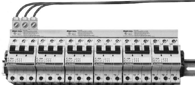
With Busbar
