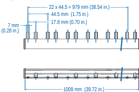
With Auxiliary Switch (1/2 pole) Spacing
