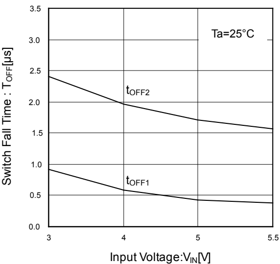
Figure 18. Switch Fall Time vs Input Voltage
