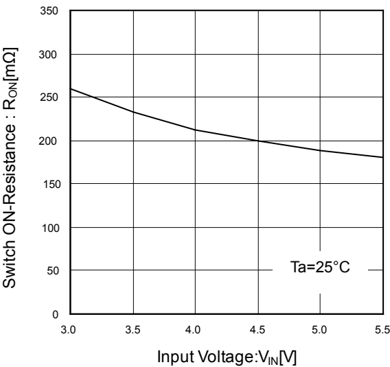
Figure 16. Switch ON-Resistance vs Input Voltage
