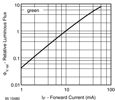
Fig. 16 - Relative Luminous Flux vs. Forward Current
