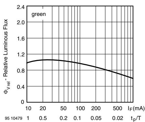
Fig. 18 - Relative Luminous Flux vs. Forward Current/Duty Cycle
