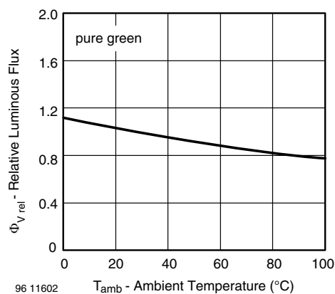
Fig. 23 - Relative Luminous Flux vs. Ambient Temperature
