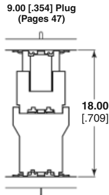
Raised Receptacle (Pages 58 and 59)
