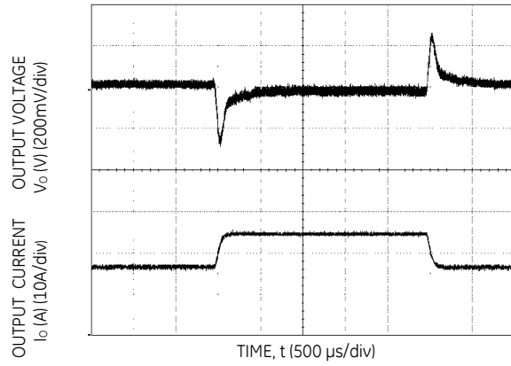
Figure 4. Typical Transient Response to 0.1A/ \mu s Step Change in Load from 50% to 75% to 50% of Full Load, C_o = 470\mu F and 48 Vdc Input.
