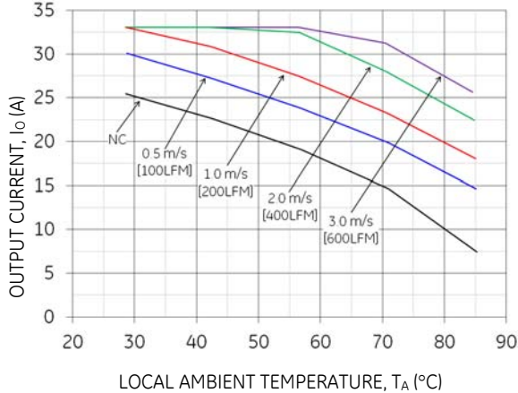
Figure 20. Output Current Derating for the Base plate QBWV033A0B-H in the Transverse Orientation; Airflow Direction from Vin(-) to Vin(+); Vin = 48V.
