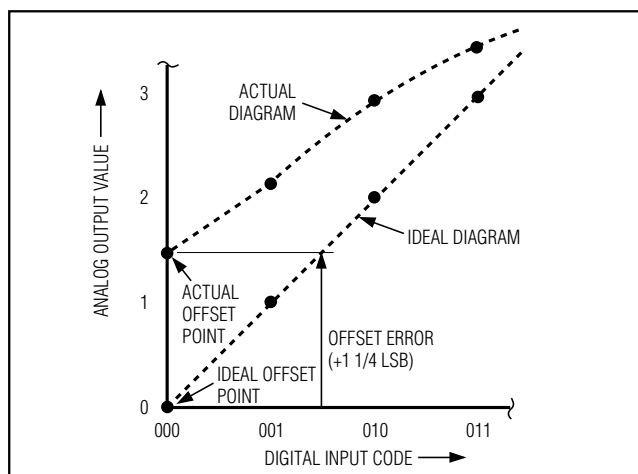
Figure 5c. Offset Error
