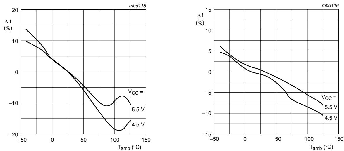
Fig 20. Frequency stability of the VCO as a function of ambient temperature with supply voltage as a parameter
