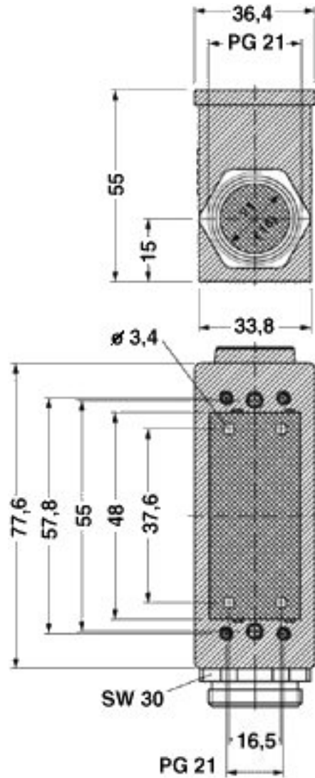
Dimensional drawing
