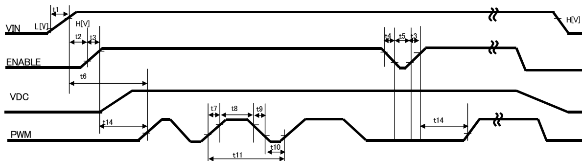
Figure 26. Input timing (after soft start)
