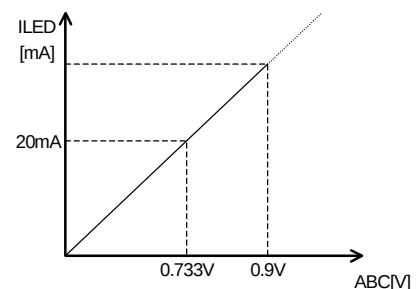
Figure 32. ILED vs ABC voltage
