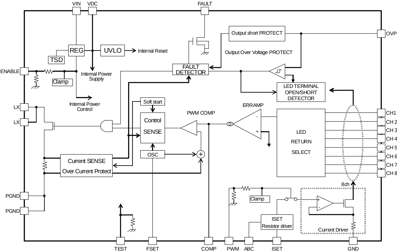
Pin number 24pin Figure 4. Block diagram
