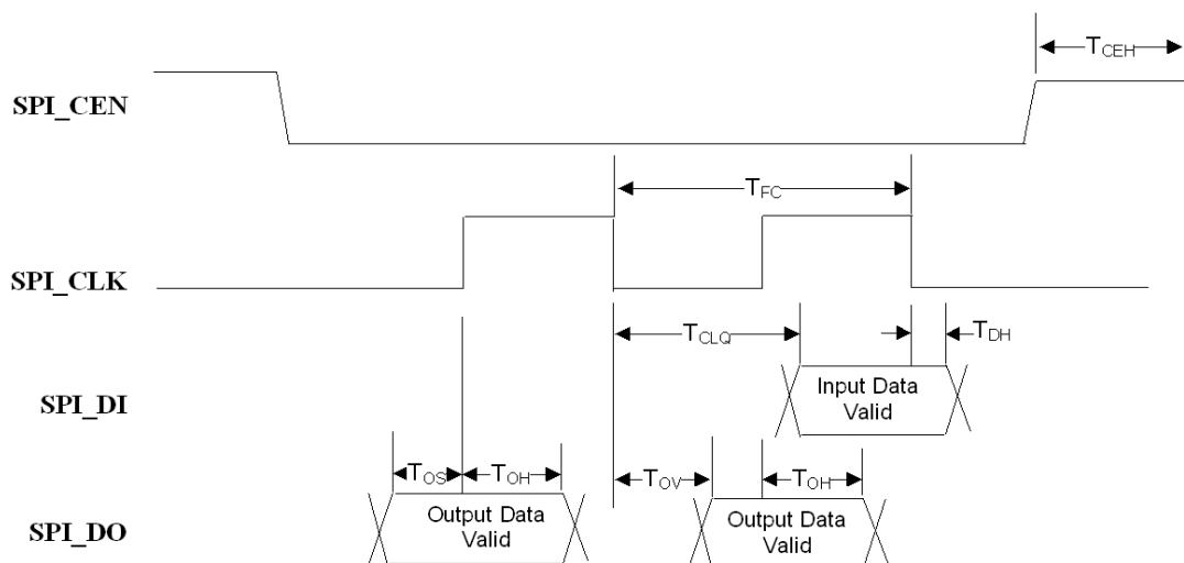
Figure 7.3 SPI Timing
