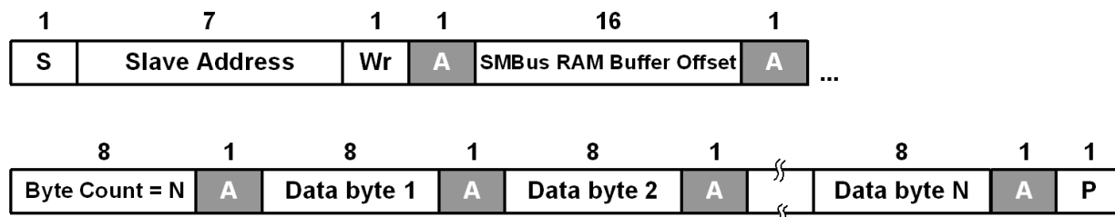
Figure 5.4 Block Write
