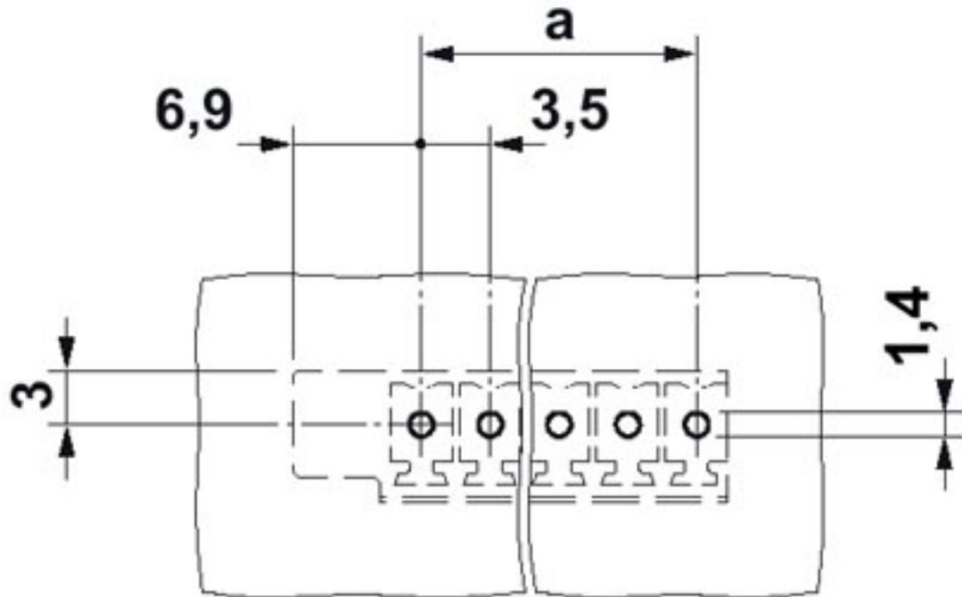
Drilling diagram
