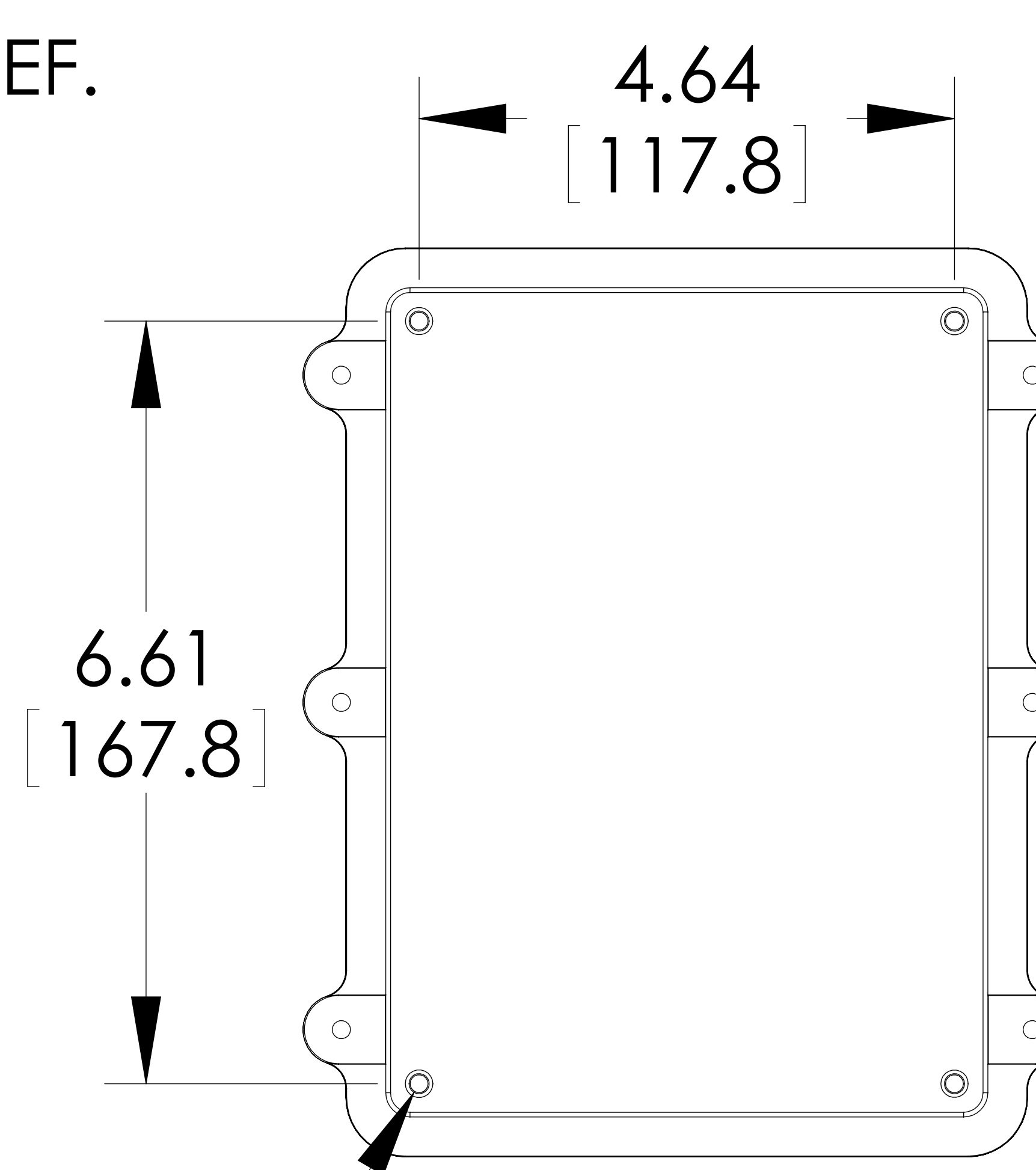
BOTTOM VIEW
