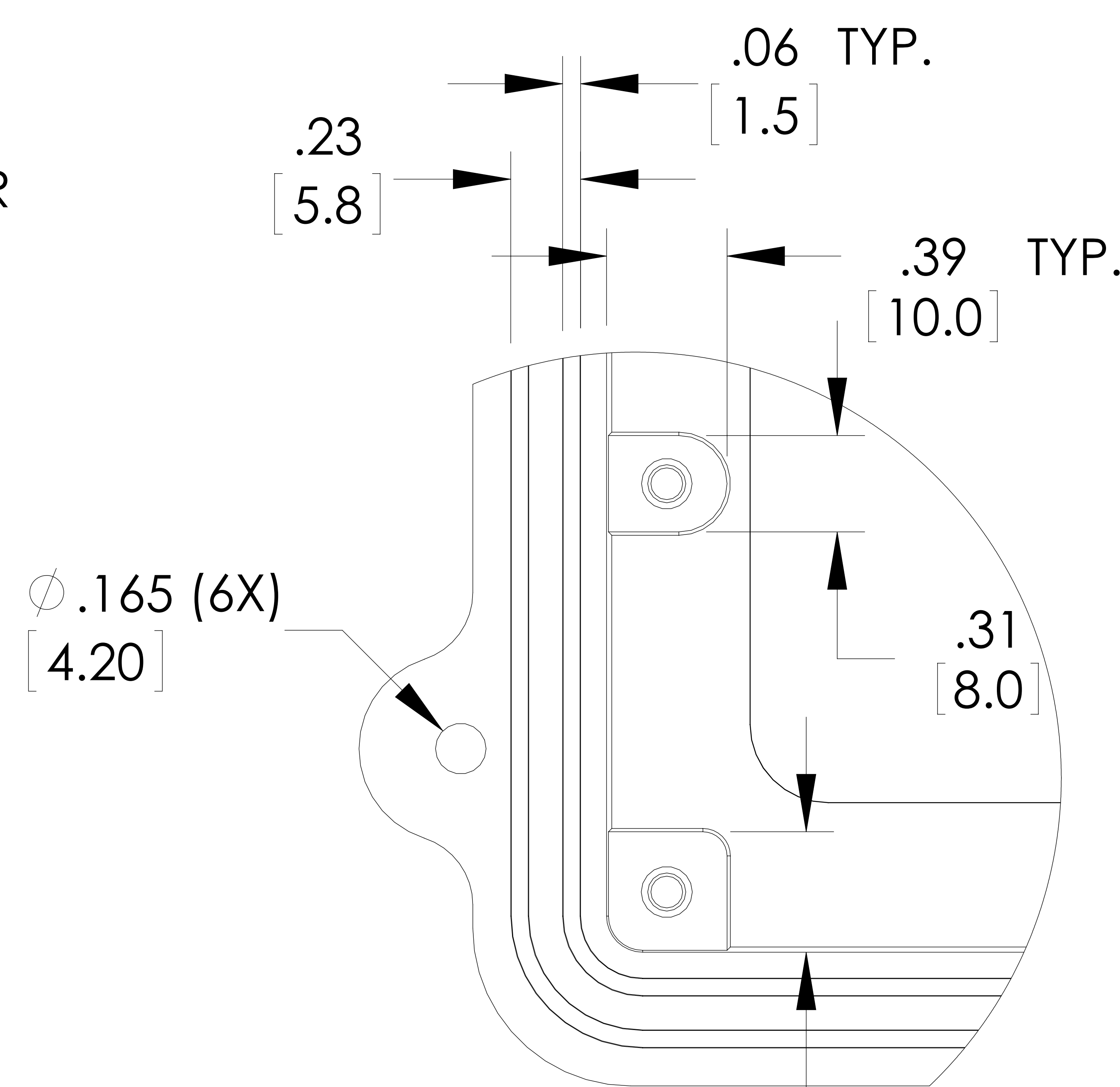
DETAIL C SCALE 4 : 1
