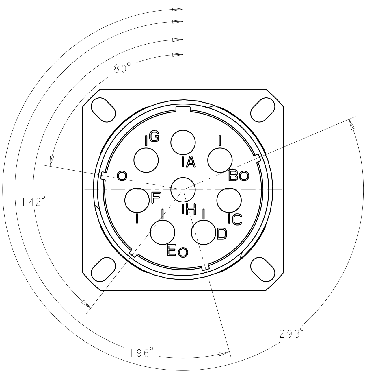
1811927-1 "N" KEY POLARIZATION
