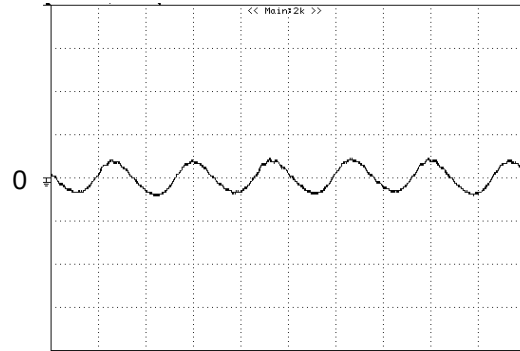
Figure 11: Input Terminal Ripple Current, i_c , at full rated output current and nominal input voltage with 12\mu H source impedance and 33\mu F electrolytic capacitor ( 200\text{ mA/div} , 1\mu s/div )
