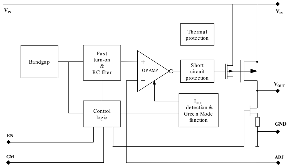
Figure 2. Block diagram (adjustable version)
