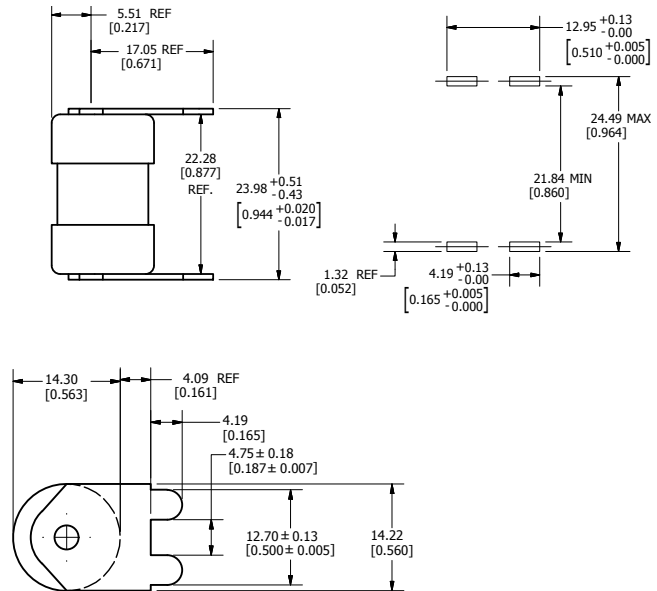
TLS-LSE Dimensions are mm (in)
