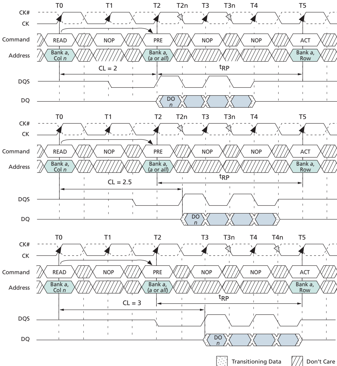
Figure 31: READ-to-PRECHARGE
