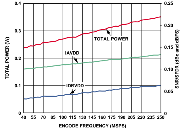
Figure 57. AD9642-250 Power and Current vs. Sample Rate
