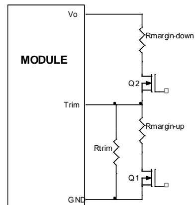
Figure 46. Circuit Configuration for margining Output voltage.
