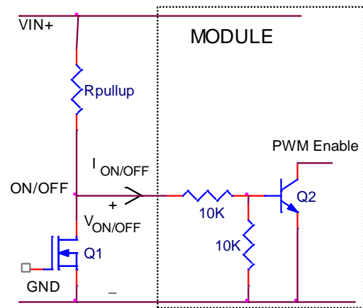
Figure 43. Circuit configuration for using negative On/Off logic.
