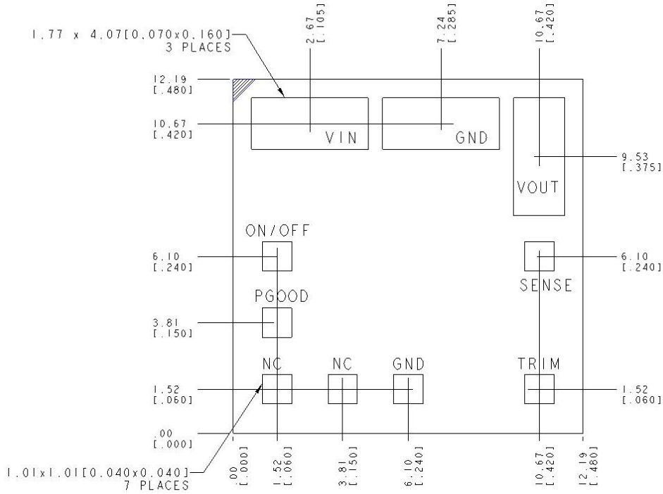
RECOMMENDED FOOTPRINT -THRU THE BOARD-
