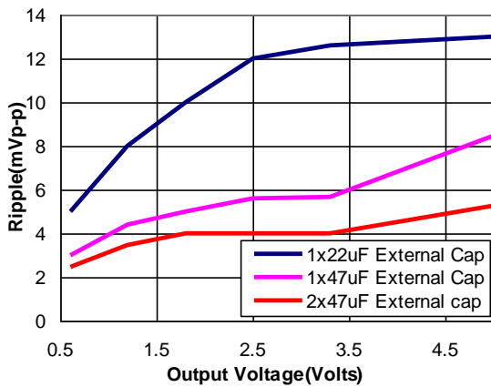
Figure 42. Output ripple voltage for various output voltages with external 1x22 µF, 1x47 µF or 2x47 µF ceramic capacitors at the output (2A load). Input voltage is 12V.
