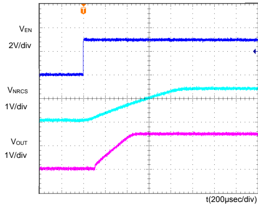
Figure 7. Waveform at Output Start
