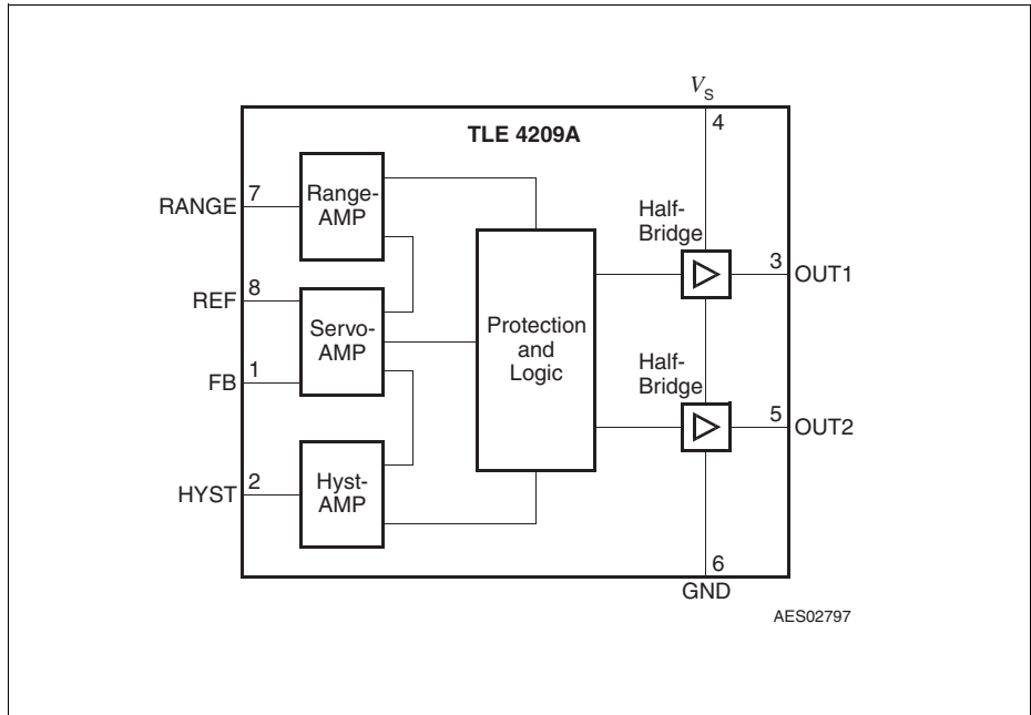
Figure 2 Block Diagram
