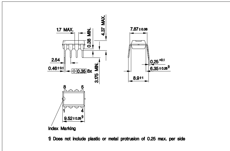
Figure 6 PG-DIP-8-4 (Plastic Dual In-line Package)
