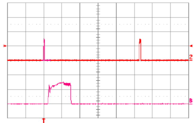
Fig. 8.0V.18: Load current (top trace, 5 A/div., 20 ms/div.) into a 10 m \Omega short circuit during restart, at V_{in} = 48V . Bottom trace (5 A/div., 1 ms/div.) is an expansion of the on-time portion of the top trace.
