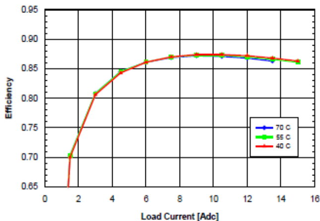
Fig. 2.0V.6: Efficiency vs. load current and ambient temperature for SQ48T/S15020 converter mounted vertically with air flowing from pin 3 to pin 1 at a rate of 200 LFM (1.0 m/s).
