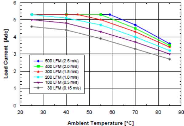
Fig. 8.0V.2: Available load current vs. ambient air temperature and airflow rates for SQ48T05080 converter with D height pins mounted horizontally with V_{in} = 48\text{ V} , air flowing from pin 3 to pin 1, and maximum FET temperature \leq 120^\circ\text{C} .
