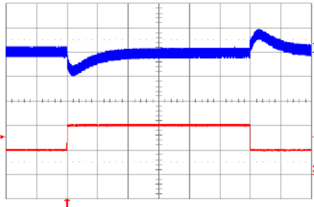
Fig. 12V.12: Output voltage response to load current step-change (1A – 2A – 1A) at V_{in} = 48V . Top trace: output voltage (200 mV/div.). Bottom trace: load current (1A/div.). Current slew rate: 5 A/ \mu s. C_o = 47\mu F tantalum + 1 \mu F ceramic. Time scale: 0.5 ms/div.
