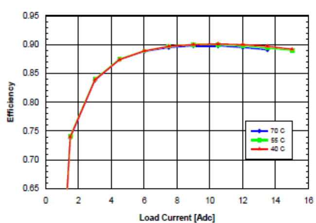
Fig. 2.5V.6: Efficiency vs. load current and ambient temperature for SQ48T/S15025 converter mounted vertically with V_{in} = 48\text{ V} and air flowing from pin 3 to pin 1 at a rate of 200 LFM (1.0 m/s).
