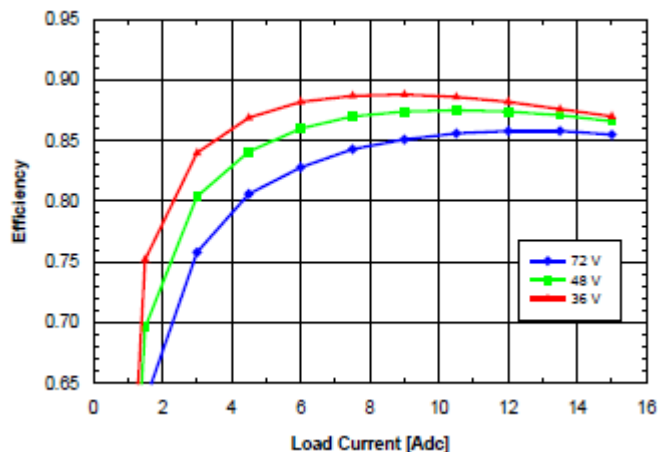
Fig. 2.0V.5: Efficiency vs. load current and input voltage for SQ48T/S15020 converter mounted vertically with air flowing from pin 3 to pin 1 at a rate of 300 LFM (1.5 m/s) and T_a = 25\text{ }^{\circ}\text{C} .
