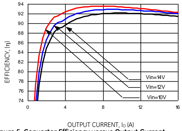
Figure 5. Converter Efficiency versus Output Current (Vout = 3.3Vdc).
