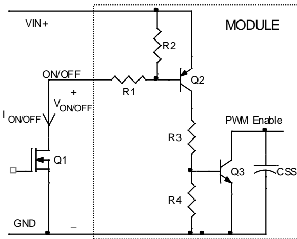
Figure 27. Circuit configuration for using positive logic On/Off.
