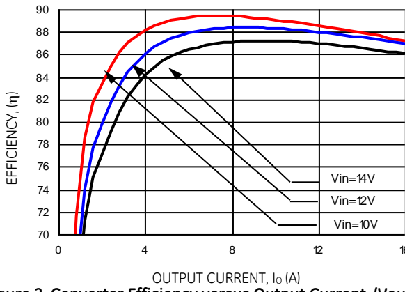
Figure 2. Converter Efficiency versus Output Current (Vout = 1.5Vdc).
