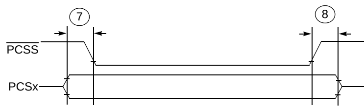
Figure 38. DSPI PCS strobe ( \overline{PCSS} ) timing
