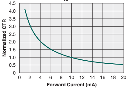
Typical Normalized CTR vs. Forward Current ( V_{CE}=0.5V )
