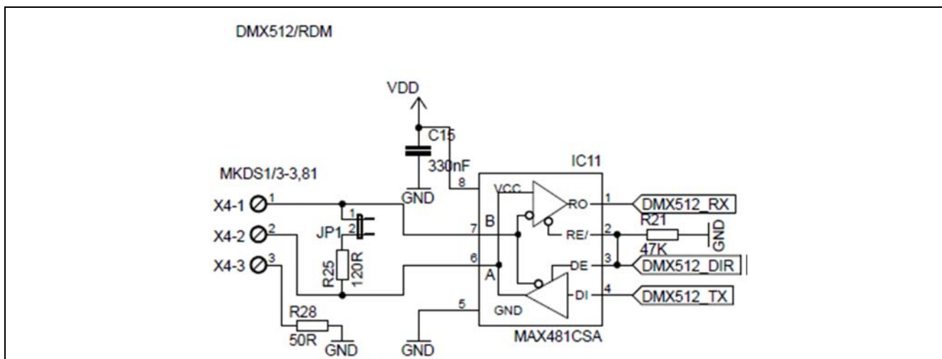
Figure 5 DMX512/RDM Circuit
