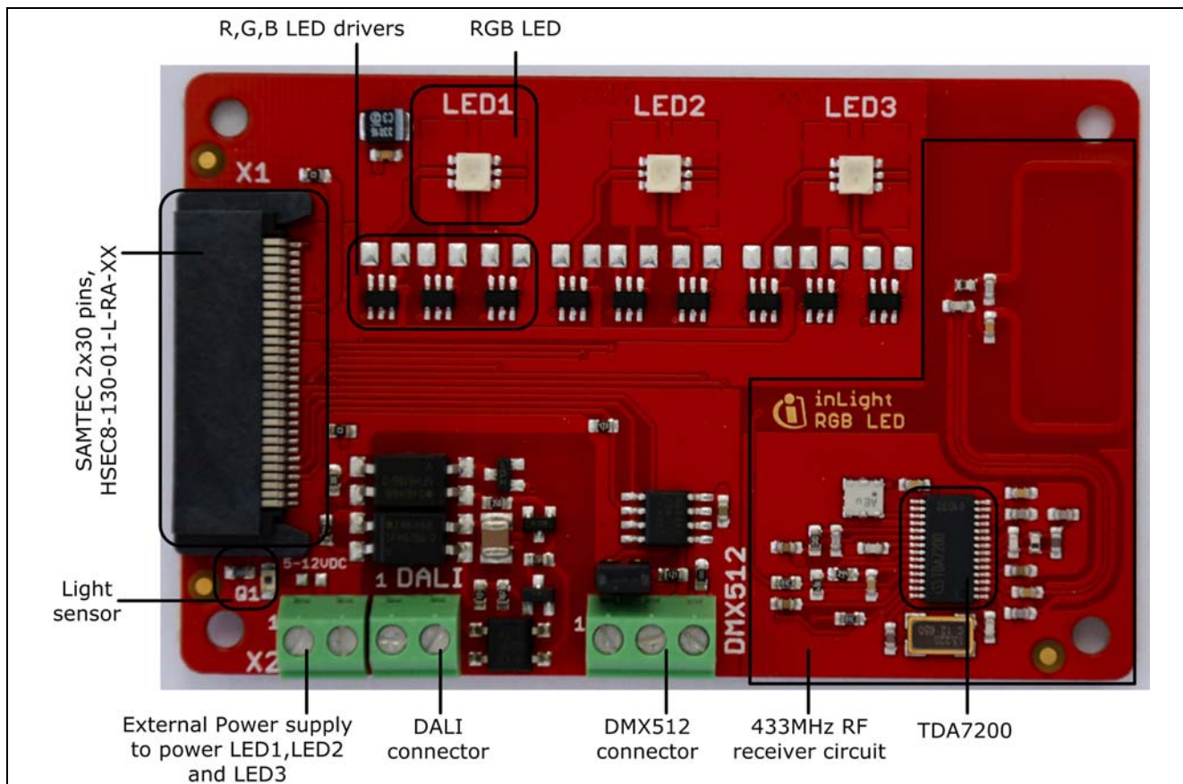
Figure 2 Colour LED Card
