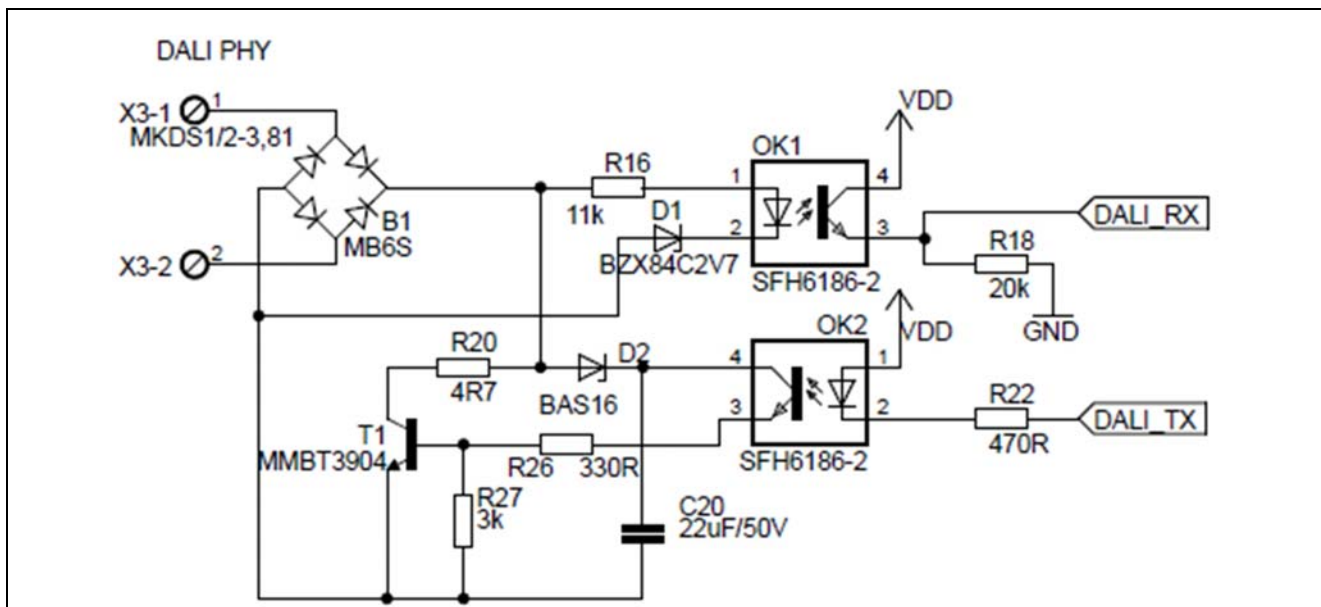
Figure 4 DALI PHY circuit
