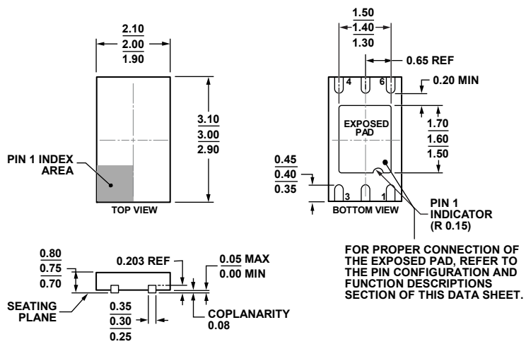
COMPLIANT TO JEDEC STANDARDS MO-229 Figure 55. 6-Lead Lead Frame Chip Scale Package [LF CSP_WD] 2.00 x 3.00 mm Body, Very Very Thin, Dual Lead (CP-6-5) Dimensions shown in millimeters
