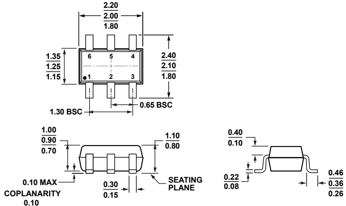
COMPLIANT TO JEDEC STANDARDS MO-203-AB Figure 54. 6-Lead Thin Shrink Small Outline Transistor Package [SC70] (KS-6) Dimensions shown in millimeters
