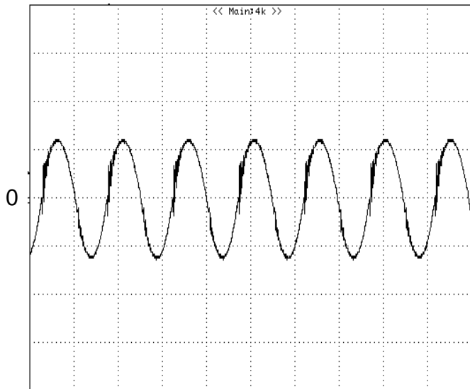
Figure 11: Input Terminal Ripple Current, i_c , at full rated output current and nominal input voltage with 12\mu\text{H} source impedance and 33\mu\text{F} electrolytic capacitor (500 mA/div, 2 µs/div)
