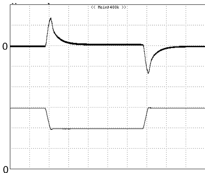
Figure 8: Output voltage response to step-change in load current (75%-50%-75% of I_{o, \text{max}} ; di/dt = 0.1\text{A}/\mu\text{s} ). Load cap: 10\mu\text{F} tantalum capacitor and 1\mu\text{F} ceramic capacitor. Top Trace: V_{\text{out}} (50mV/div, 200us/div), Bottom Trace: I_{\text{out}} (5A/div). Scope measurement should be made using a BNC cable (length shorter than 20 inches). Position the load between 51 mm to 76 mm (2 inches to 3 inches) from the module
