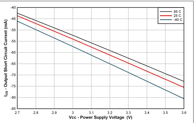
Figure 2. Output Short-Circuit Current vs Power Supply Voltage
