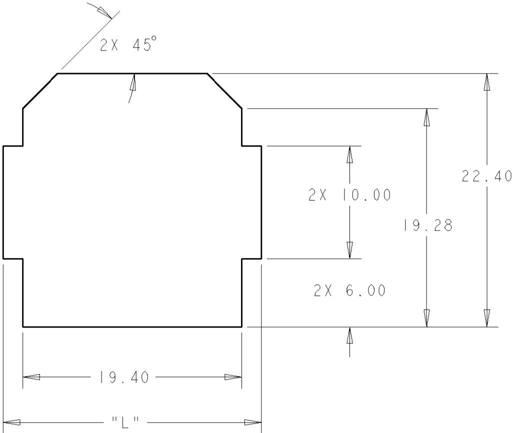
PANEL CUT-OUT
