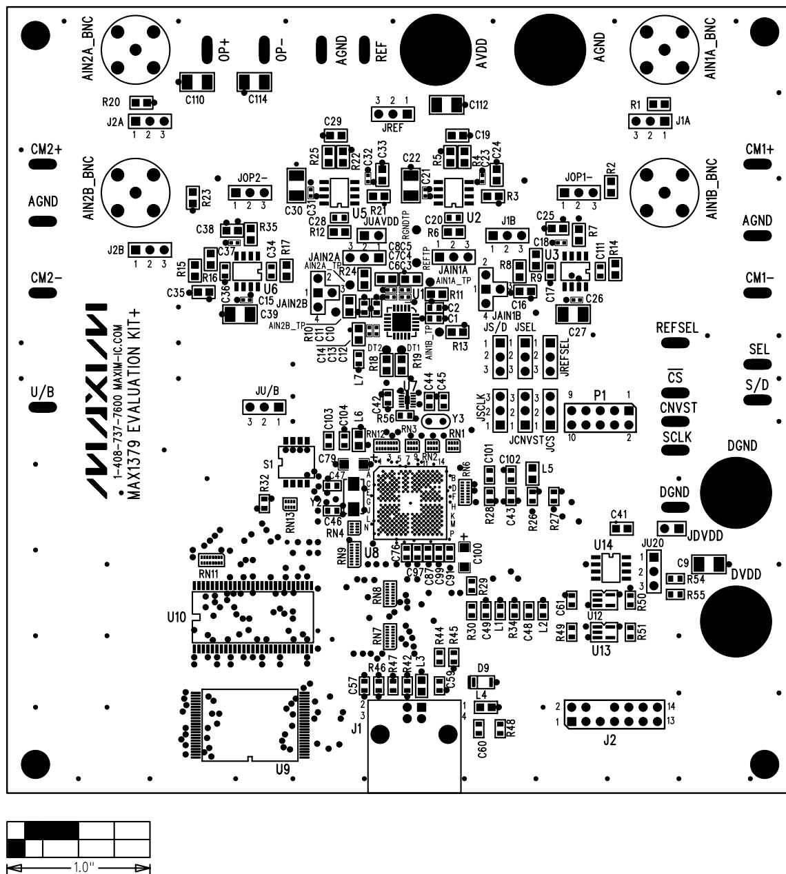
Figure 3. MAX1379 EV Kit Component Placement Guide—Top Silkscreen
