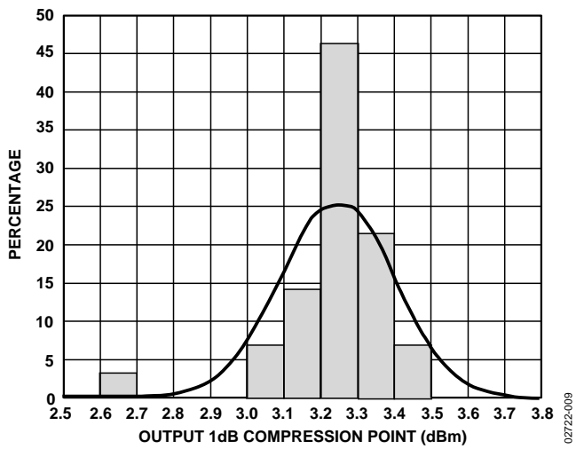
Figure 10. Distribution of P_{1dB} , V_S = 3 V, T_A = 25^\circ\text{C} , f = 2.2 GHz
