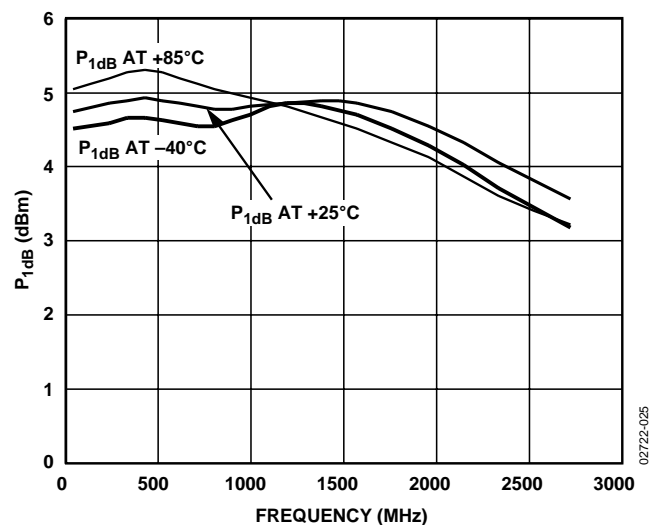
Figure 26. P_{1dB} vs. Frequency, V_S = 5 V, T_A = -40^\circ\text{C} , +25^\circ\text{C} , and +85^\circ\text{C}
