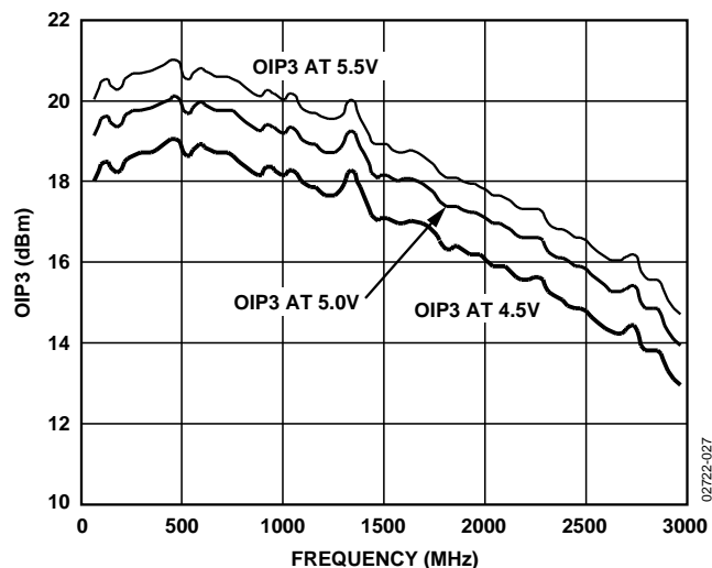
Figure 28. OIP3 vs. Frequency, V_S = 4.5\text{ V} , 5\text{ V} , and 5.5\text{ V} , T_A = 25^\circ\text{C}
