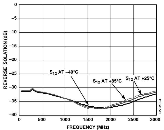
Figure 25. Reverse Isolation vs. Frequency, V_S = 5 V, T_A = -40^\circ\text{C} , +25^\circ\text{C} , and +85^\circ\text{C}
