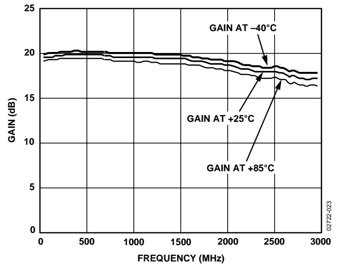
Figure 24. Gain vs. Frequency, V_S = 5 V, T_A = -40^\circ\text{C} , +25^\circ\text{C} , and +85^\circ\text{C}
