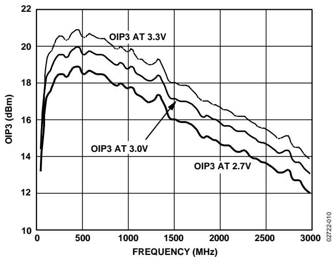
Figure 11. OIP3 vs. Frequency, V_S = 2.7 V, 3 V, and 3.3 V, T_A = 25^\circ\text{C}
