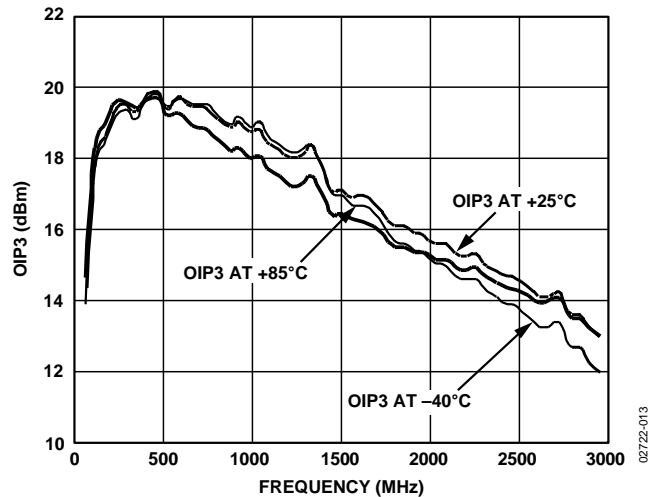
Figure 14. OIP3 vs. Frequency, V_S = 3 V, T_A = -40^\circ\text{C} , +25^\circ\text{C} , and +85^\circ\text{C}
