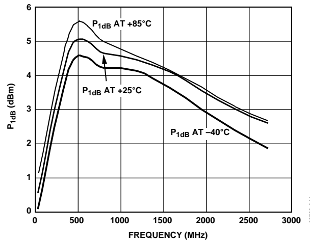
Figure 12. P_{1dB} vs. Frequency, V_S = 3 V, T_A = -40^\circ\text{C} , +25^\circ\text{C} , and +85^\circ\text{C}
