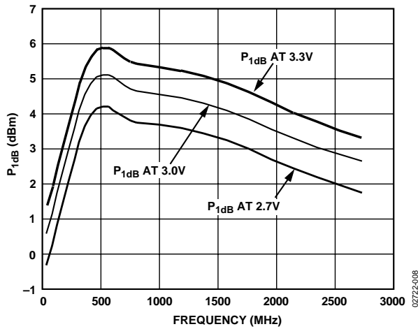
Figure 9. P_{1dB} vs. Frequency, V_S = 2.7 V, 3 V, and 3.3 V, T_A = 25^\circ\text{C}
