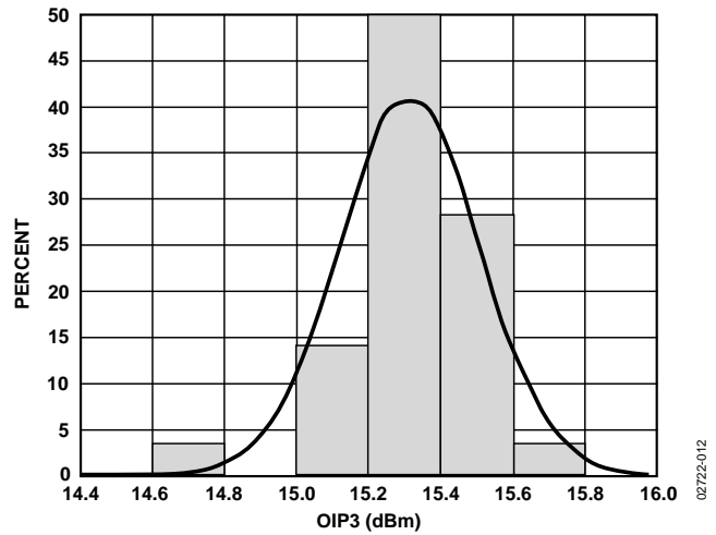
Figure 13. Distribution of OIP3 , V_S = 3 V, T_A = 25^\circ\text{C} , f = 2.2 GHz
