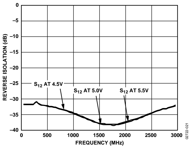
Figure 22. Reverse Isolation vs. Frequency, V_S = 4.5 V, 5 V, and 5.5 V, T_A = 25^\circ\text{C}
