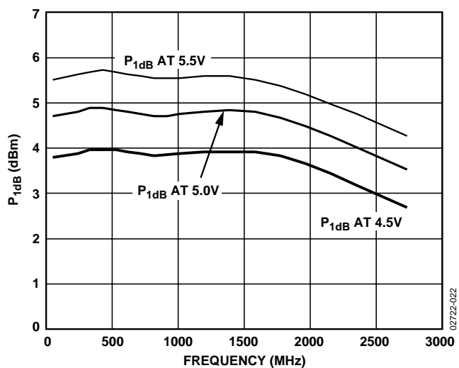
Figure 23. P_{1dB} vs. Frequency, V_S = 4.5 V, 5 V, and 5.5 V, T_A = 25^\circ\text{C}
