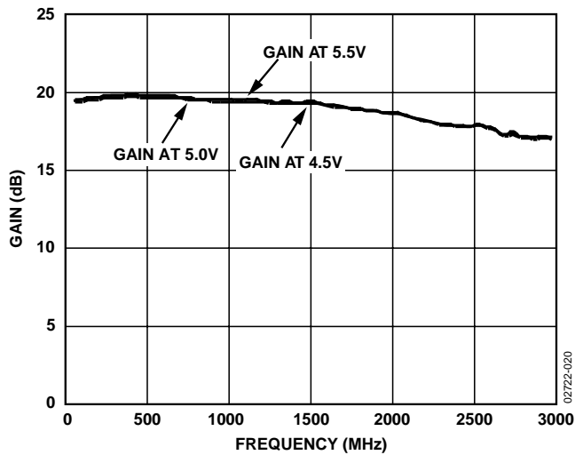
Figure 21. Gain vs. Frequency, V_S = 4.5 V, 5 V, and 5.5 V, T_A = 25^\circ\text{C}
