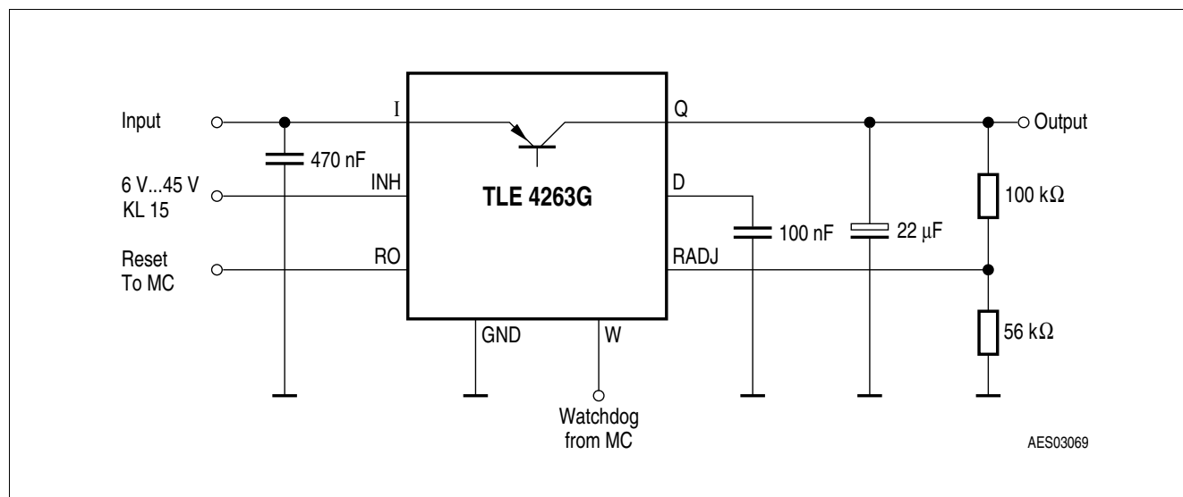
Figure 3 Application circuit
