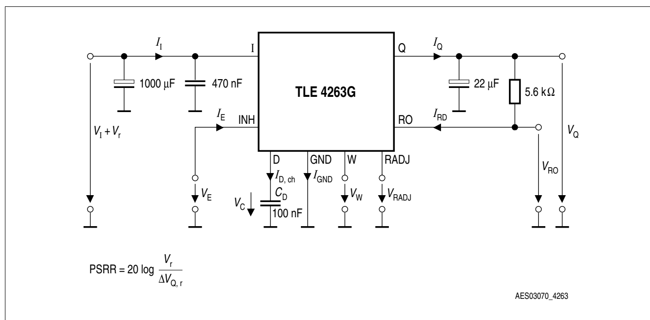
Figure 4 Test circuit
