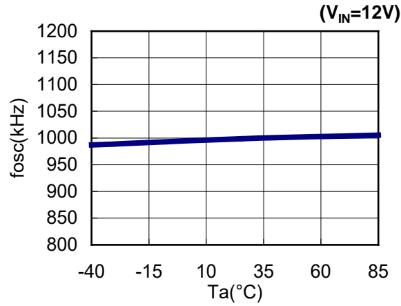
7) Oscillator Frequency(ver.G,H)
