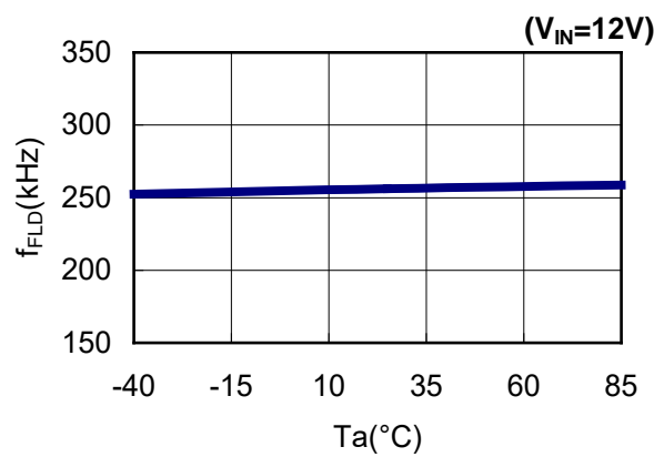
11) Fold-Back Frequency(ver.G,H)
