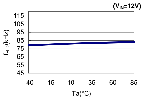
9) Fold-Back Frequency(ver.C,D)
