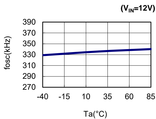
5)Oscillator Frequency(ver.C,D)
