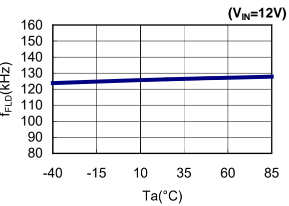
10) Fold-Back Frequency(ver.E,F)
