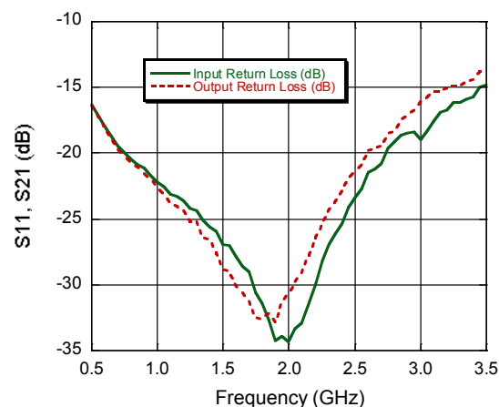
Return Loss
