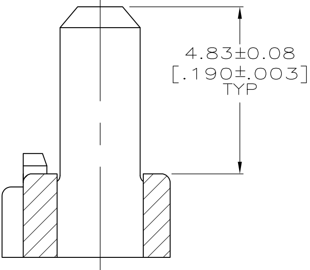
SECTION Z-Z
