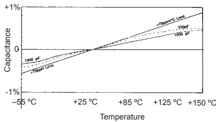
Capacitance Change vs. Temperature
