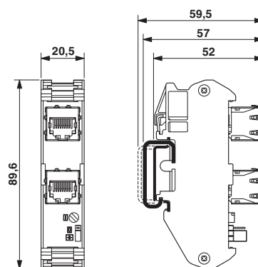
Dimensional drawing
